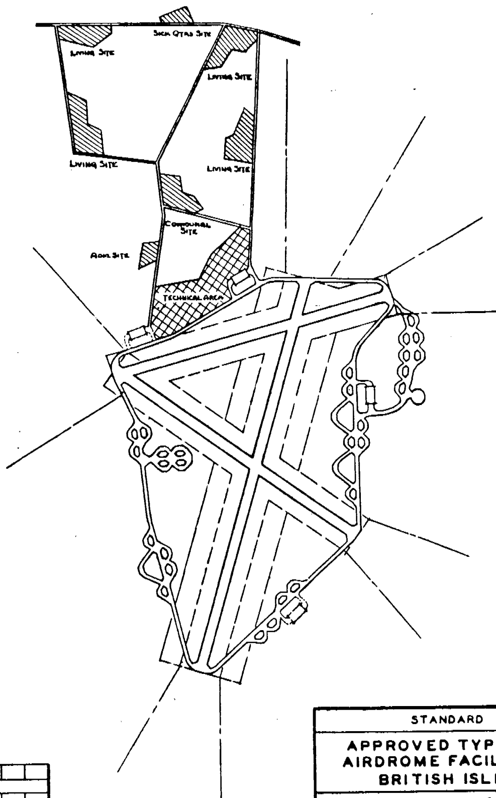
TYPICAL AIRDROME LAYOUT IN BRITISH ISLES
